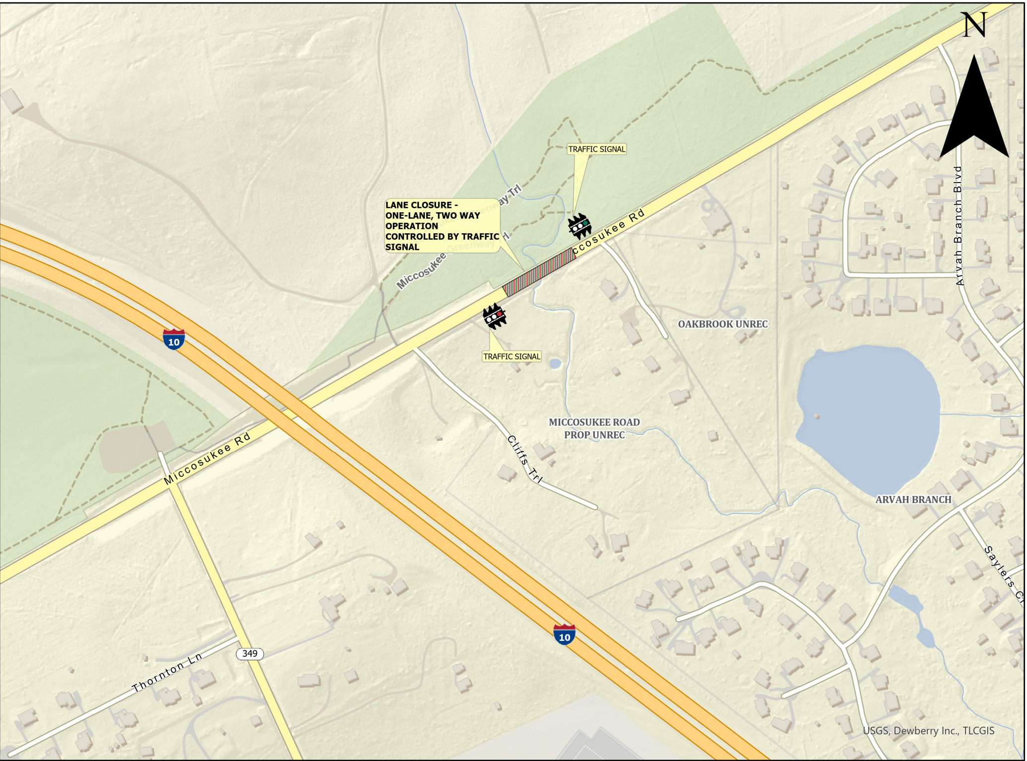
Miccosukee Road Bridge Replacement - One-Lane, Two-Way Operation
